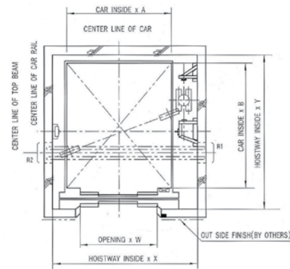
4 PANEL CENTER OPEN
