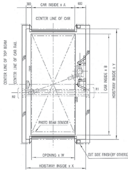
PLAN OF HOISTWAY
