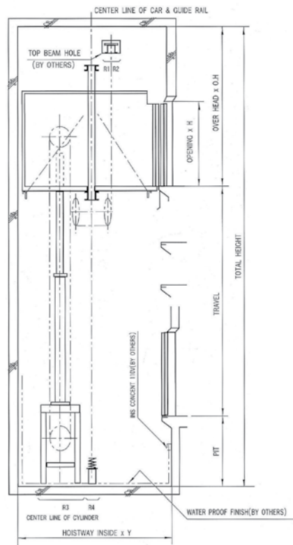
SECTION OF HOISTWAY
